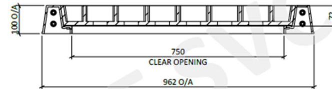
SECTION X-X
