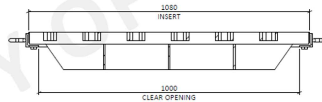
SECTION Y-Y
