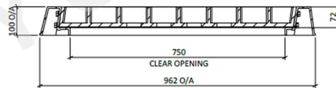
SECTION Y-Y
