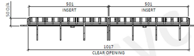
SECTION X-X
