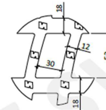
PATTERN DETAIL NOT TO SCALE
