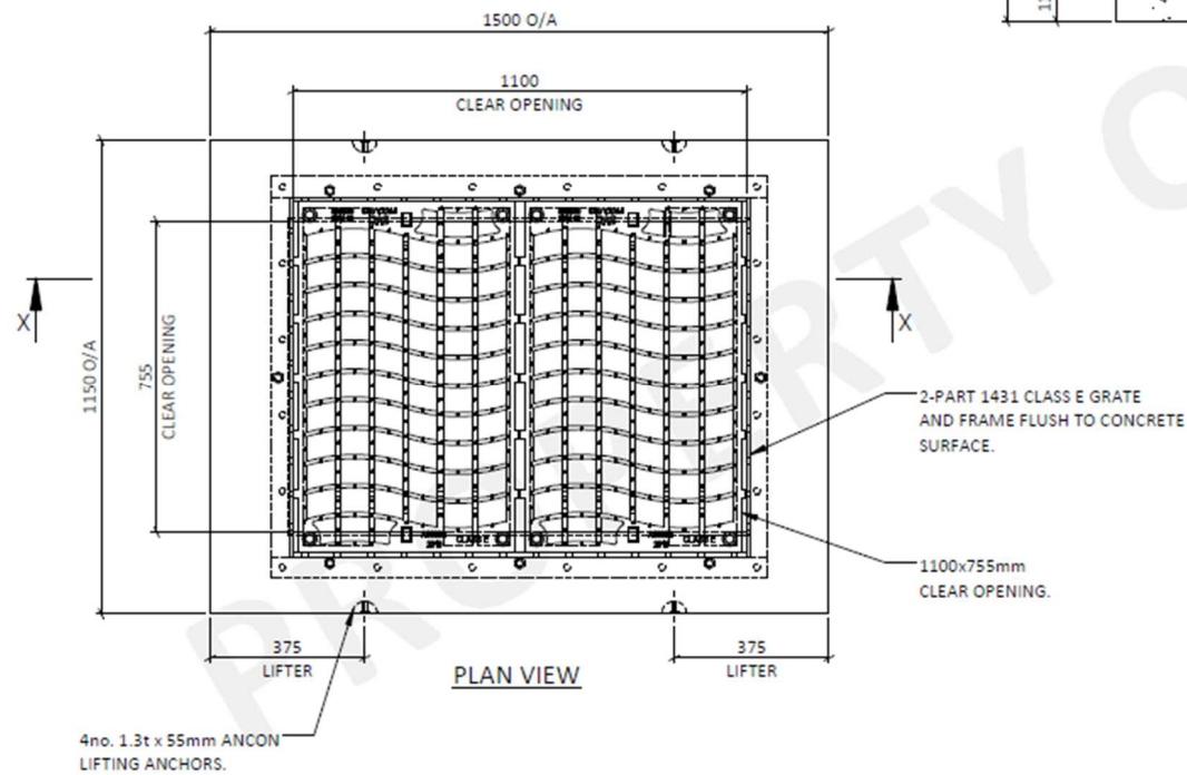
LIFTING DIAGRAM
