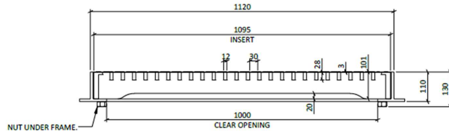
SECTION X-X
