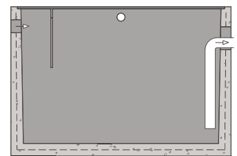
PETROL & OIL
